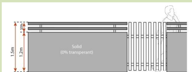
Example: Combination fencing, 0% transparent to 1.2m then 50% transparent from 1.2 to 1.5.
