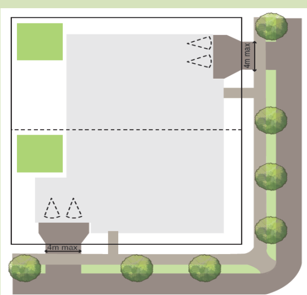
Example: Dual occupancy - corner lot, individual driveways.
