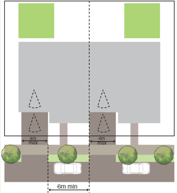
Example: Dual occupancy - individual driveways are separated.
