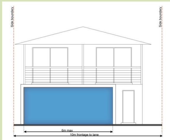
Example: Dwelling house – lot frontage less than 12.5m adjoining a laneway.
