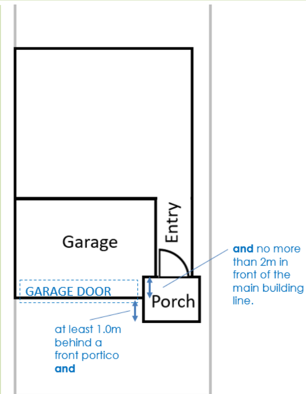
Carport/Garage openings relative to the location of the front porch/portico or the like and the main building line.
